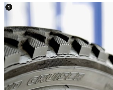
Fatigue cracks
