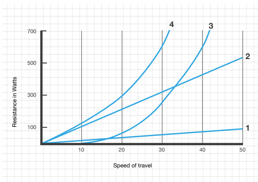
Resistance force on a bicycle
